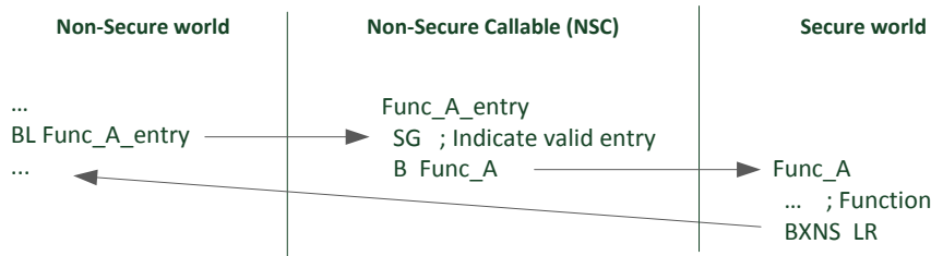
Figure 5: Software flow when Non-Secure program call a function (e.g. API) in Secure side
