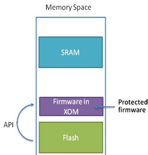
Figure 2: XOM technique for firmware protection
