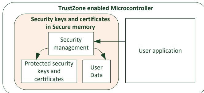
Figure 11: TrustZone technology for protection of sensitive data
