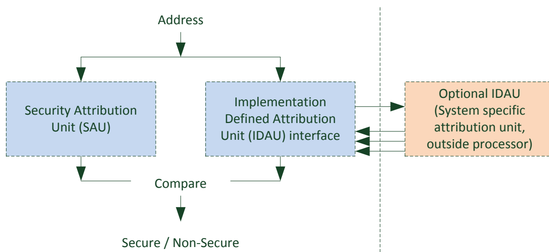
Figure 4: Security attribute defined by optional SAU and IDAU
