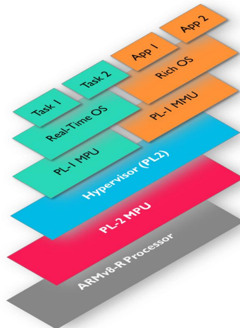
Figure 2: Second privilege layer in the ARMv8-R supports hardware assisted virtualization
