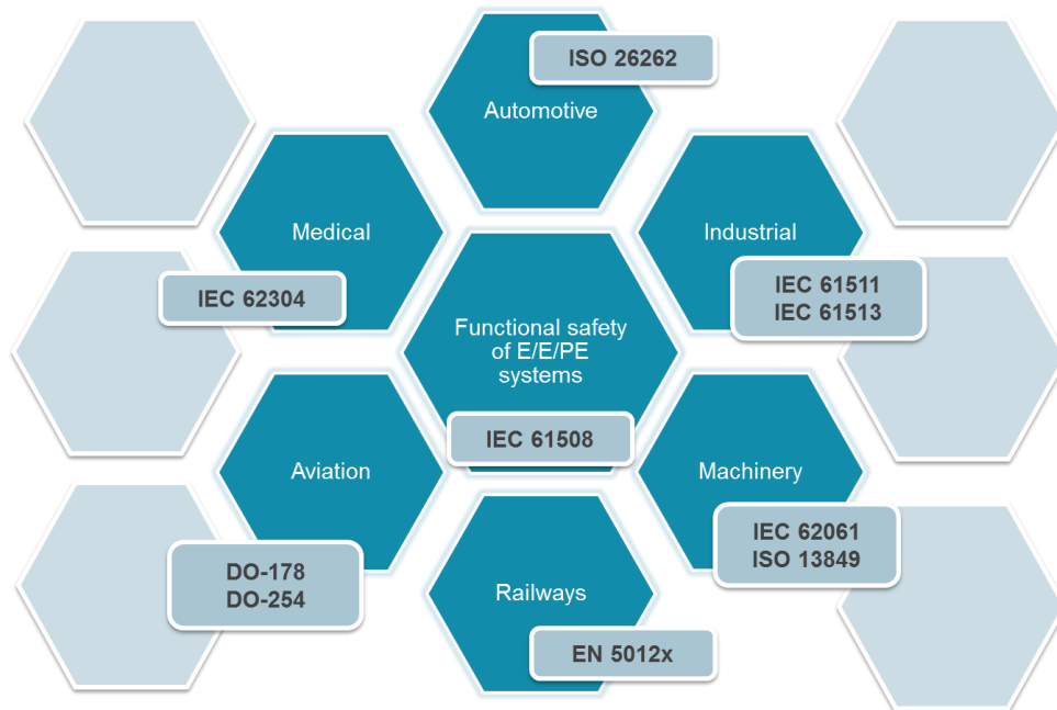
Figure 1: Main functional safety and related standards
