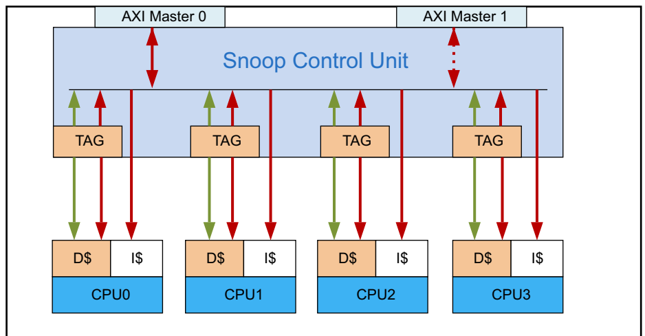
Figure 3-23 Snoop Control Unit
