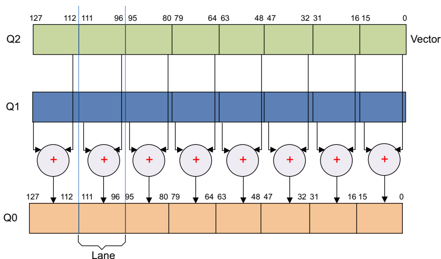
Figure 3-10 8-lane 16-bit integer add operation
