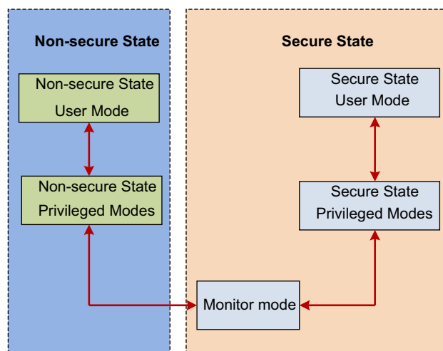
Figure 3-21 Non-secure and Secure states
