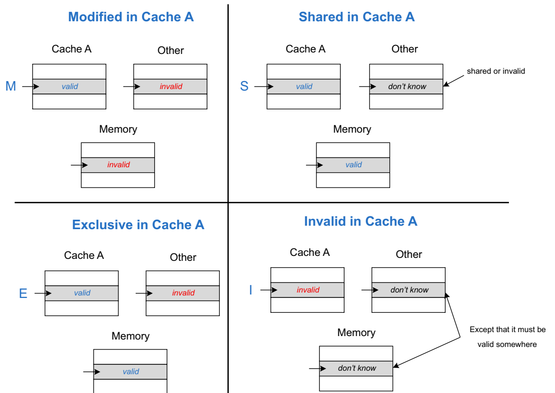
Figure 3-22 MESI state in memory and cache
