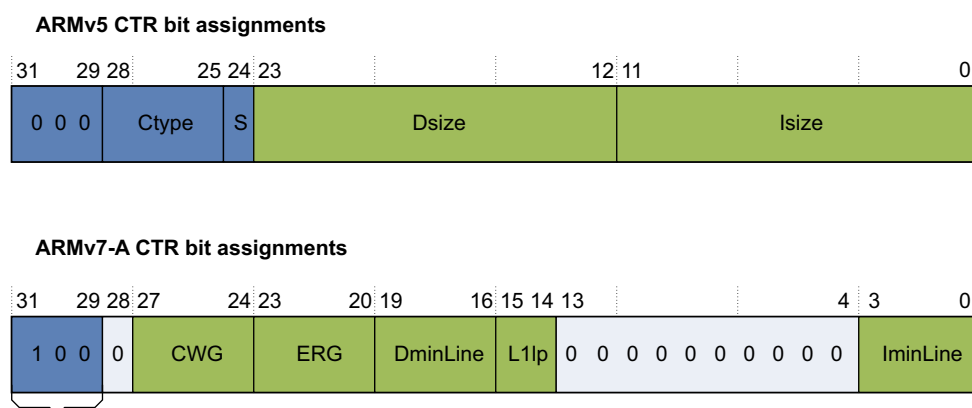
Figure 3-2 Bit assignments of Cache Type Register in ARMv5 and ARMv7-A
