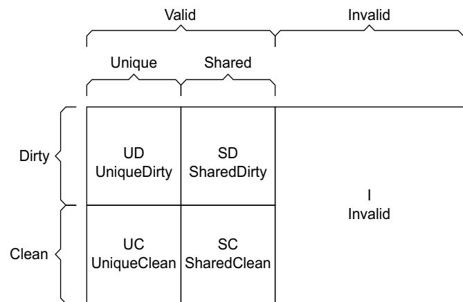
Figure D1-2 ACE cache state model
